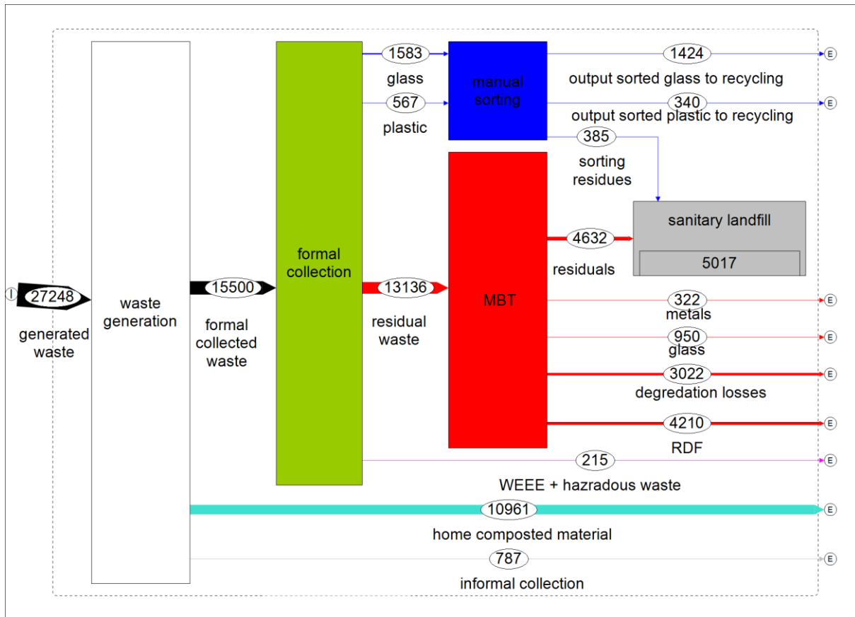
Figure 9: Material flow diagram of scenario 1a - Recycling low [gl, pl]
